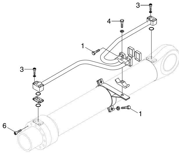
BOOM CYLINDER
