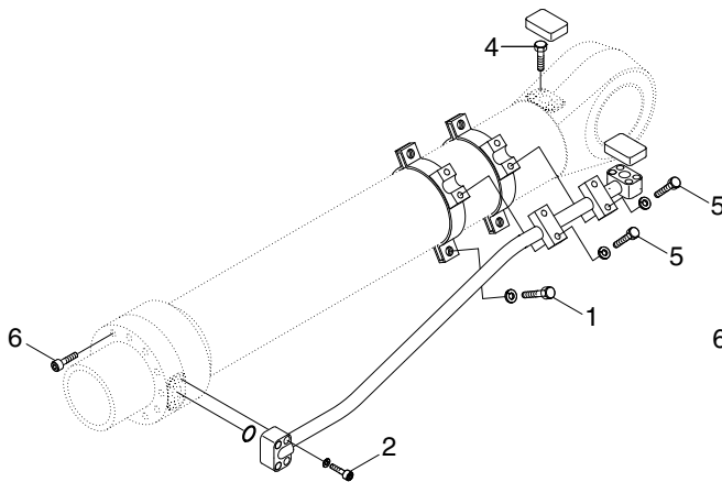
ARM CYLINDER
