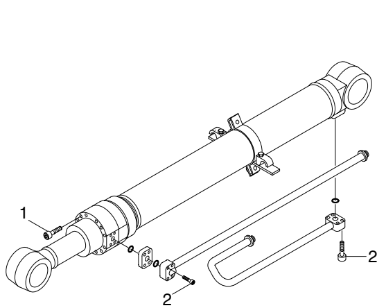
BOOM CYLINDER
