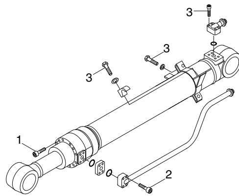
ARM CYLINDER
