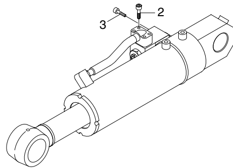
DOZER CYLINDER
