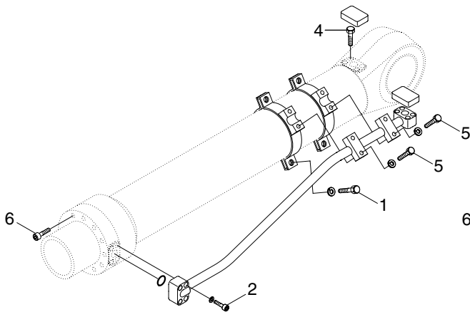
ARM CYLINDER
