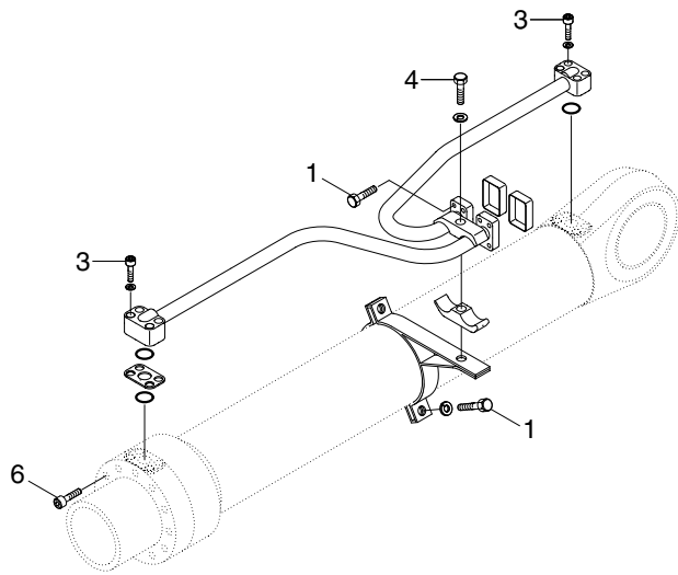
BOOM CYLINDER
