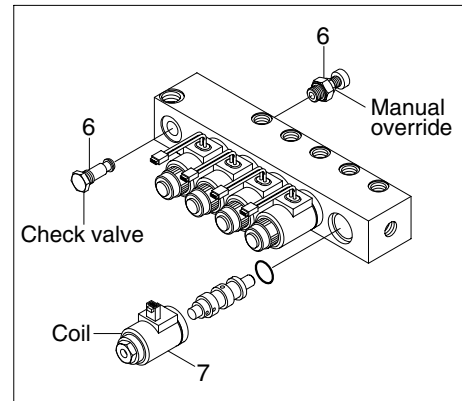
Solenoid valve
