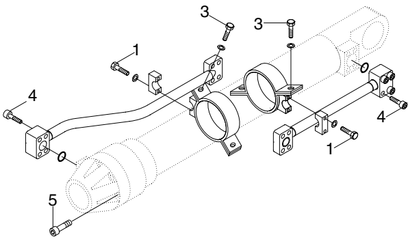
BUCKET CYLINDER
