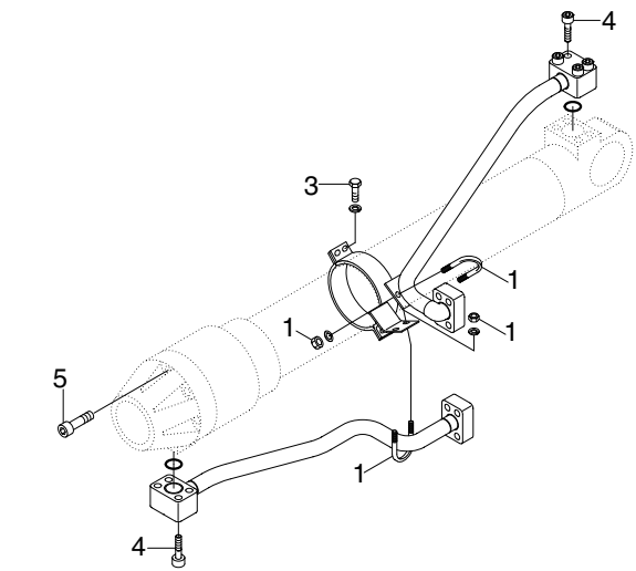
BOOM CYLINDER
