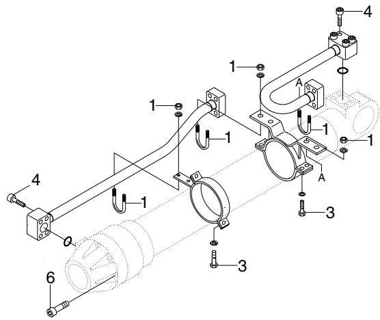
ARM CYLINDER
