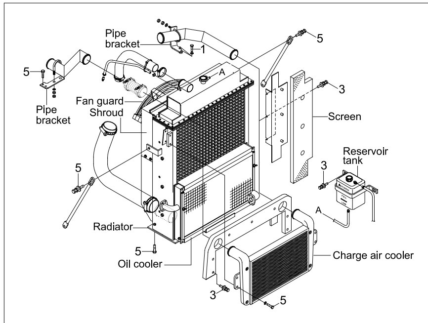
VIEW A
