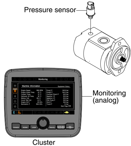
Cluster
