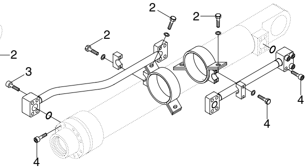
BUCKET CYLINDER
