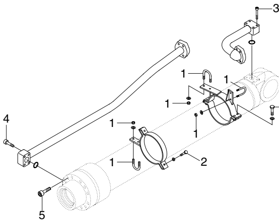
ARM CYLINDER
