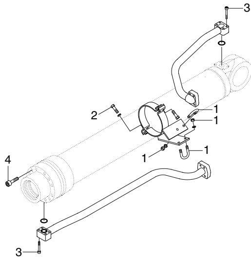
BOOM CYLINDER
