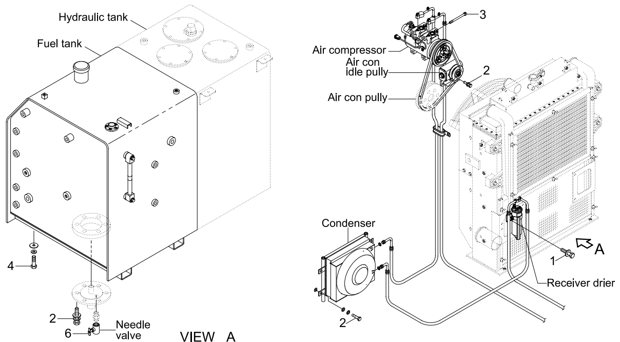
VIEW A
