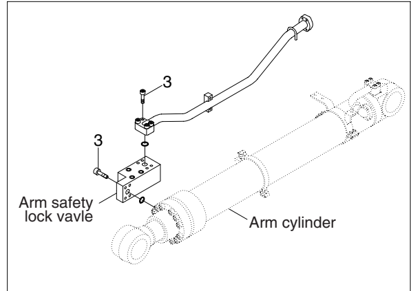
Arm safety lock system
