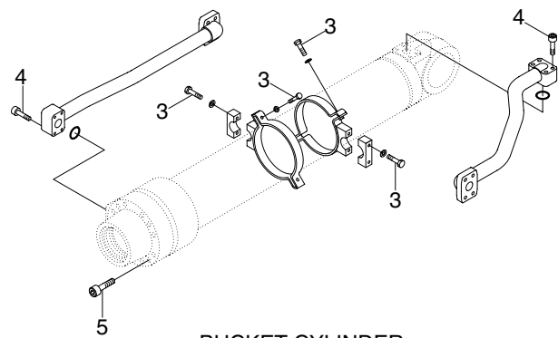
BUCKET CYLINDER
