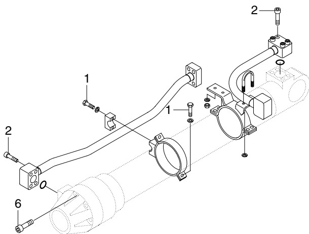
ARM CYLINDER
