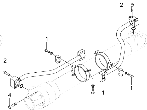
BUCKET CYLINDER
