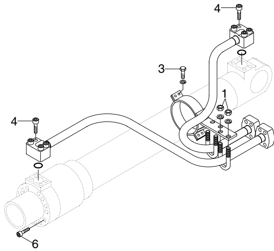
BOOM CYLINDER
