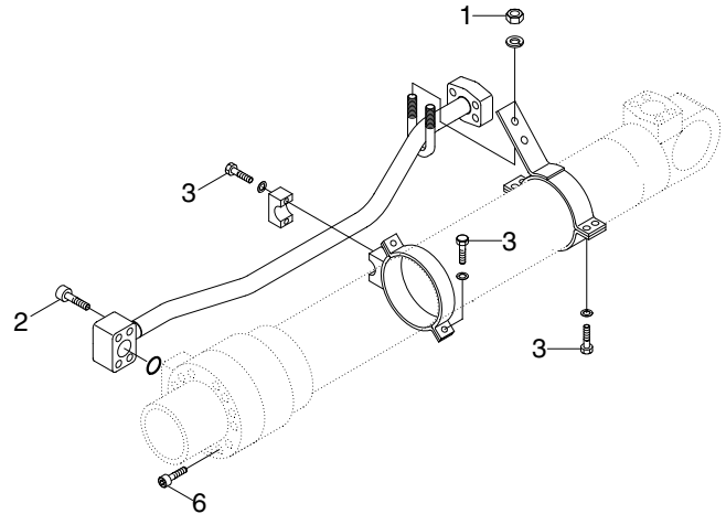
ARM CYLINDER
