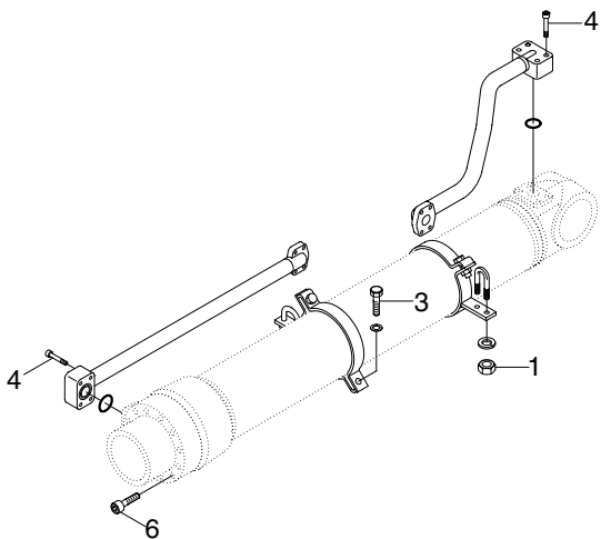
BUCKET CYLINDER
