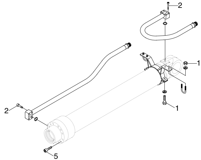
BUCKET CYLINDER (LONG REACH)
