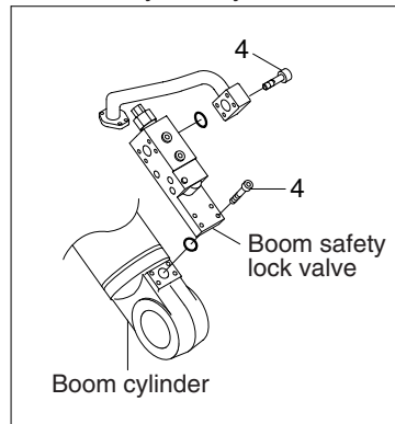
Boom safety lock system
