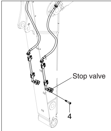
Double acting attachment piping
