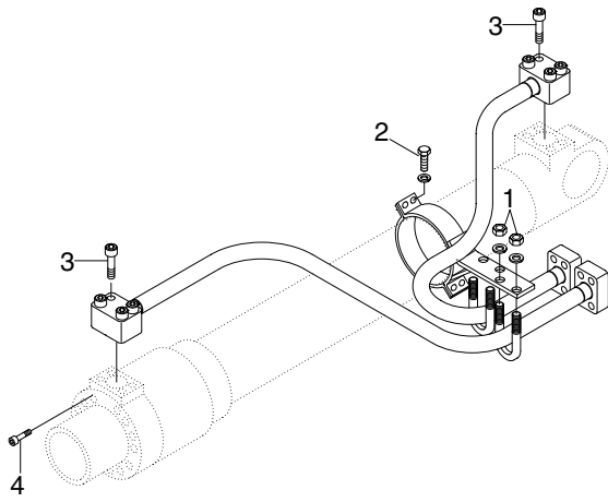
BOOM CYLINDER
