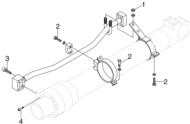
ARM CYLINDER
