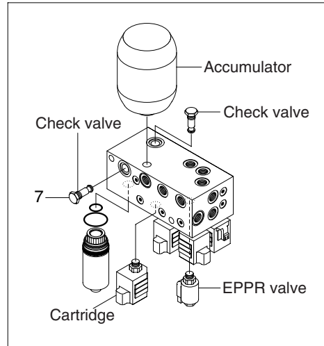
Solenoid valve
