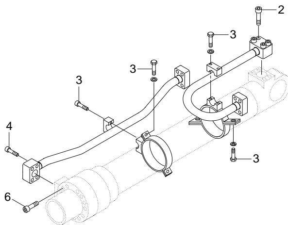
ARM CYLINDER
