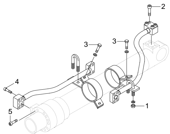
BUCKET CYLINDER
