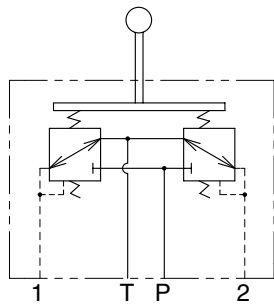
Hydraulic circuit
