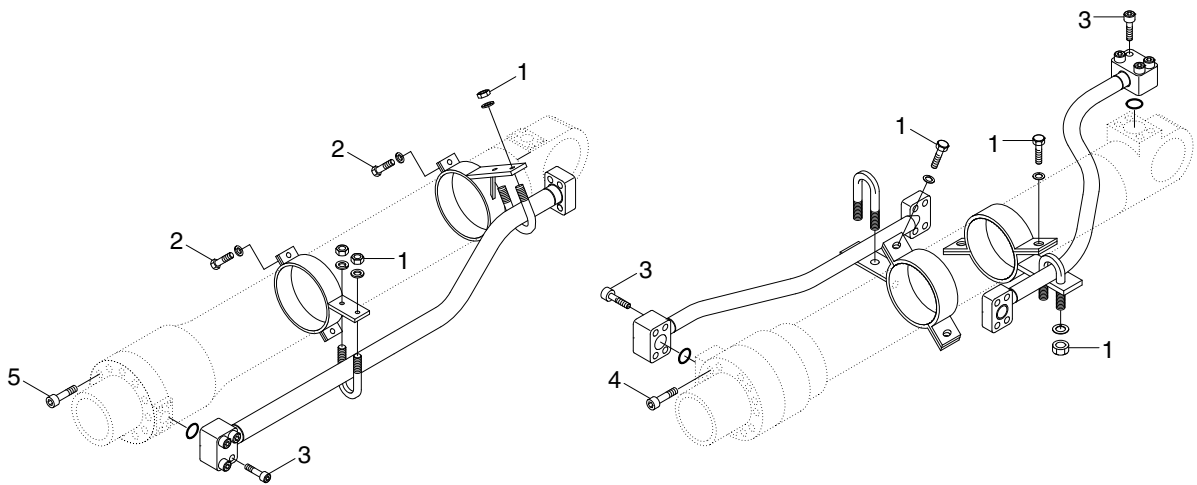
ARM CYLINDER
