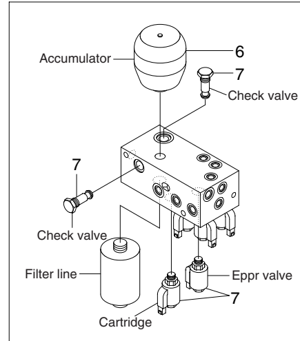
Solenoid valve
