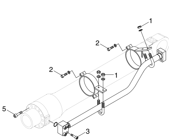
ARM CYLINDER
