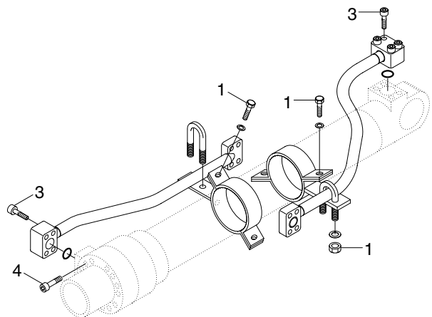
BUCKET CYLINDER
