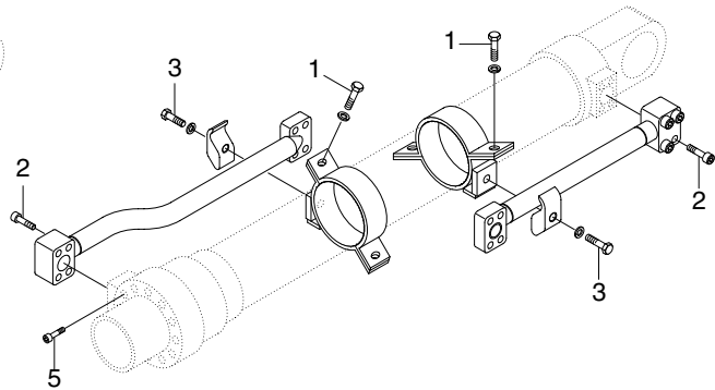
BUCKET CYLINDER
