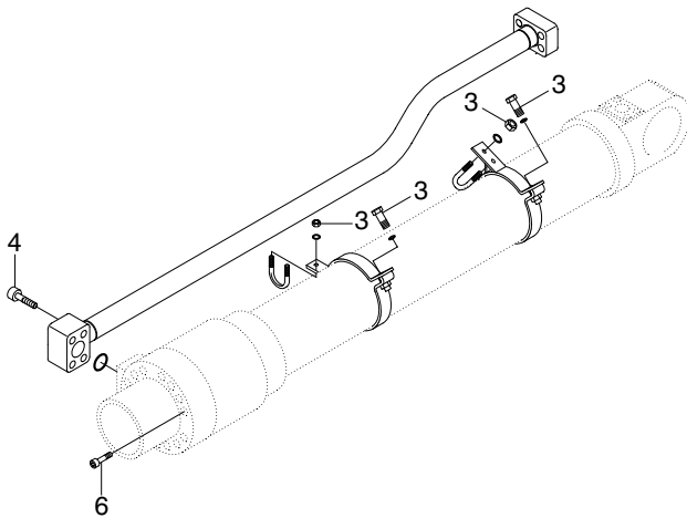
ARM CYLINDER
