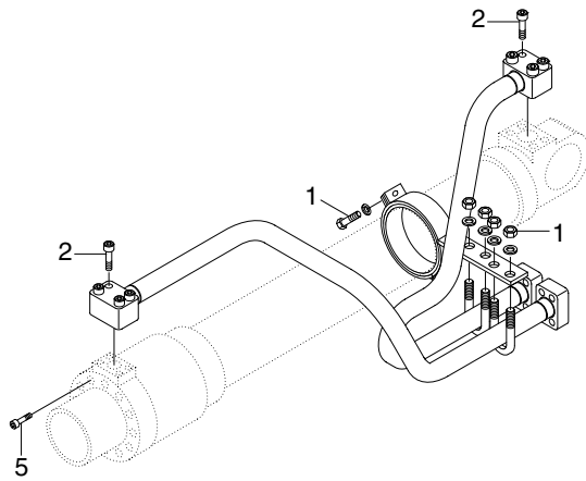
BOOM CYLINDER
