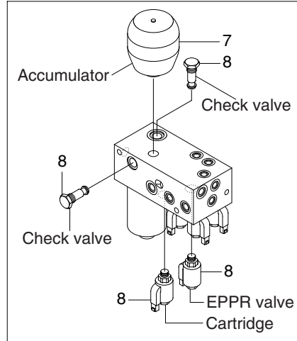
Solenoid valve
