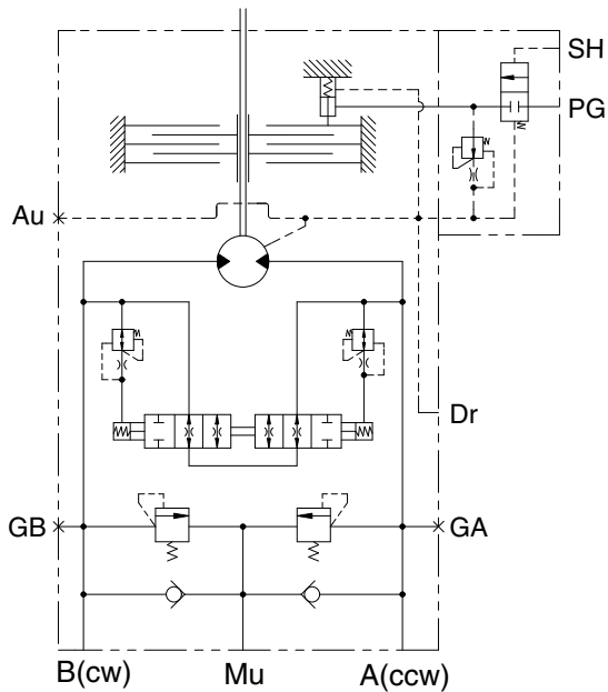
Hydraulic circuit
