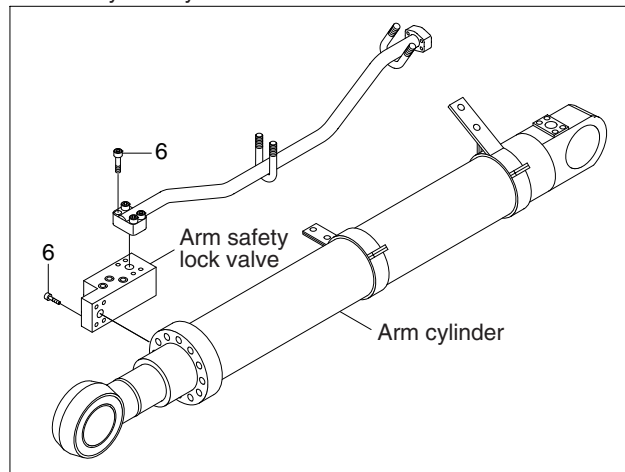
Arm safety lock system
