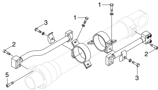
BUCKET CYLINDER
