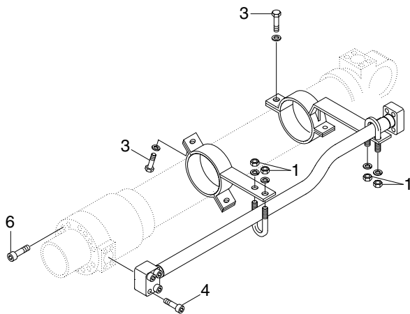
ARM CYLINDER
