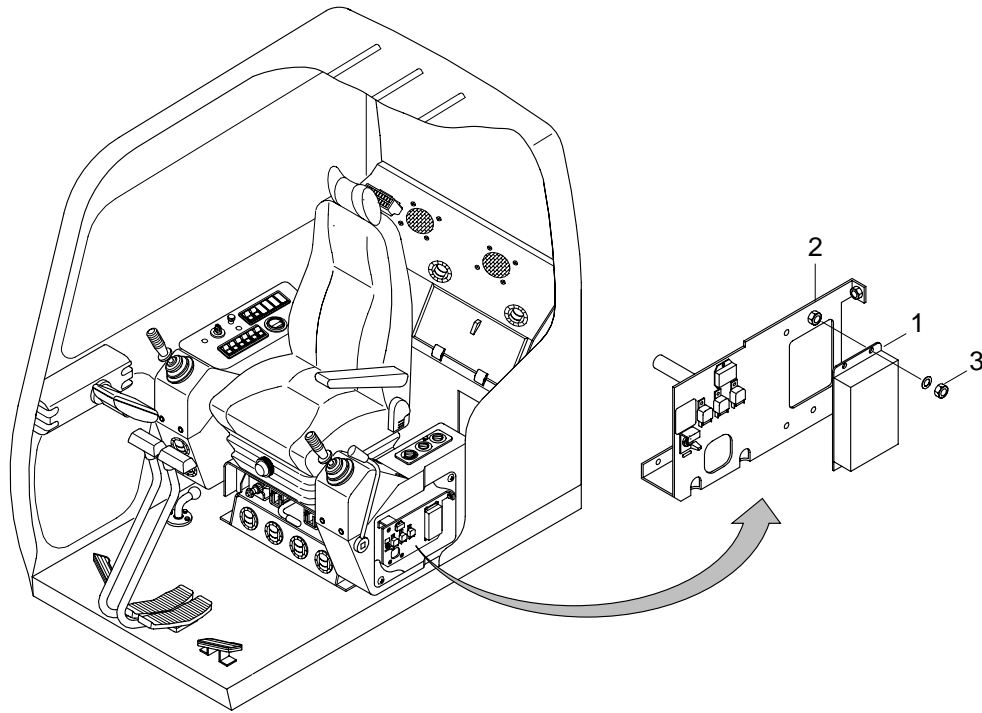
1 CPU controller 2 Controller mounting bracket 3 Nut
