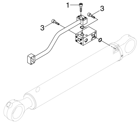
DOZER BLADE CYLINDER
