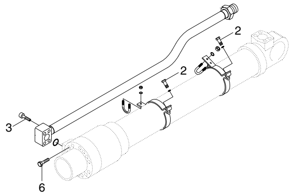
ARM CYLINDER
