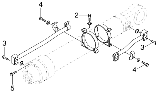
BUCKET CYLINDER
