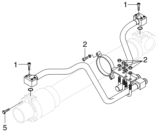
BOOM CYLINDER
