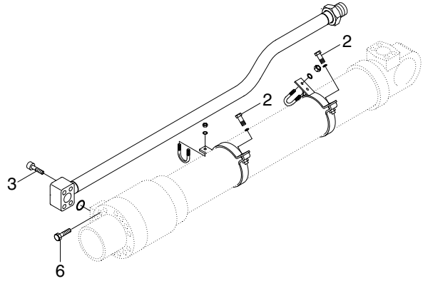
ARM CYLINDER
