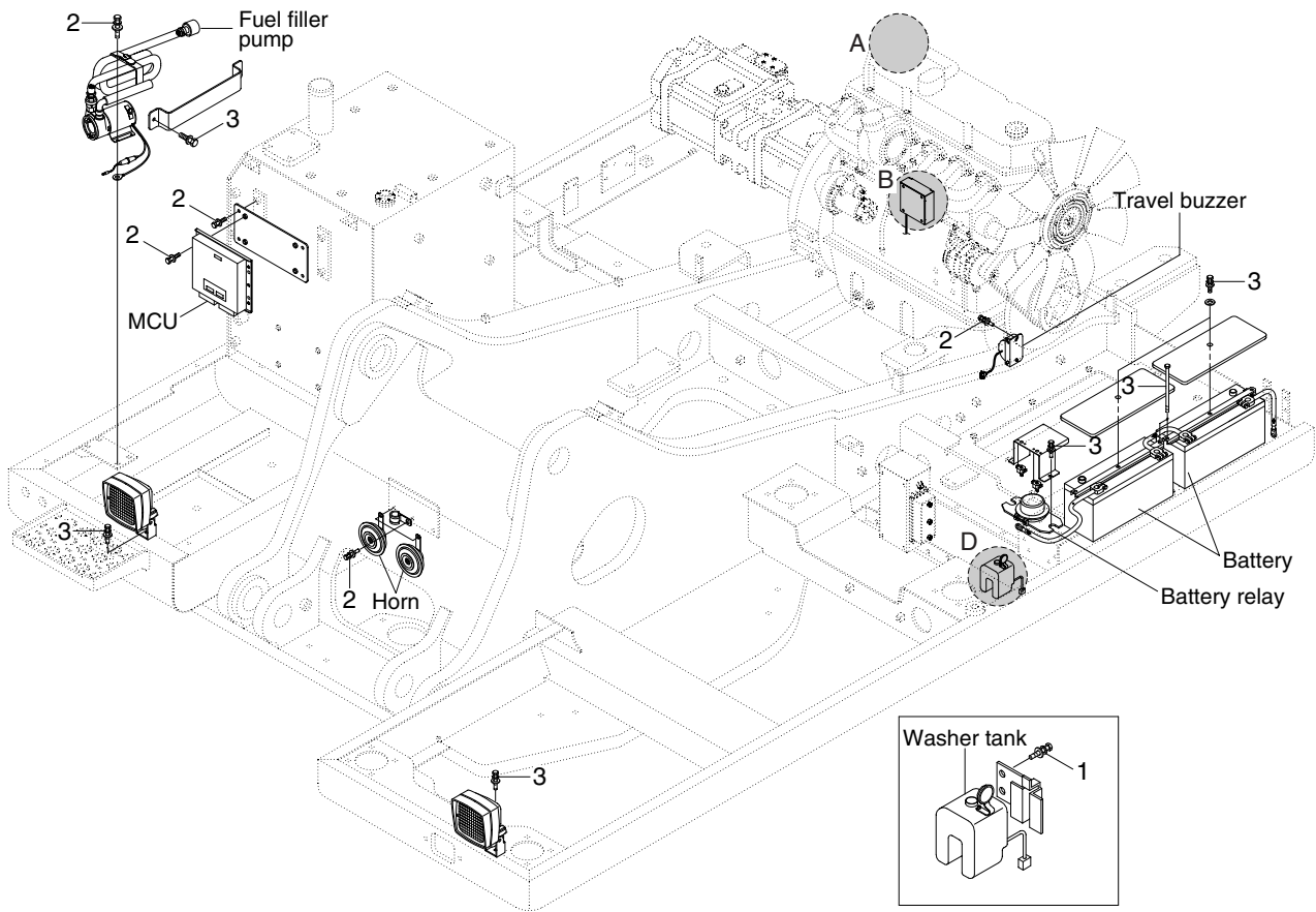
DETAIL C
