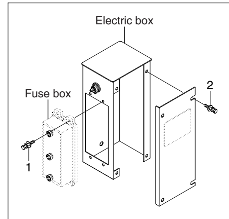
VIEW A
