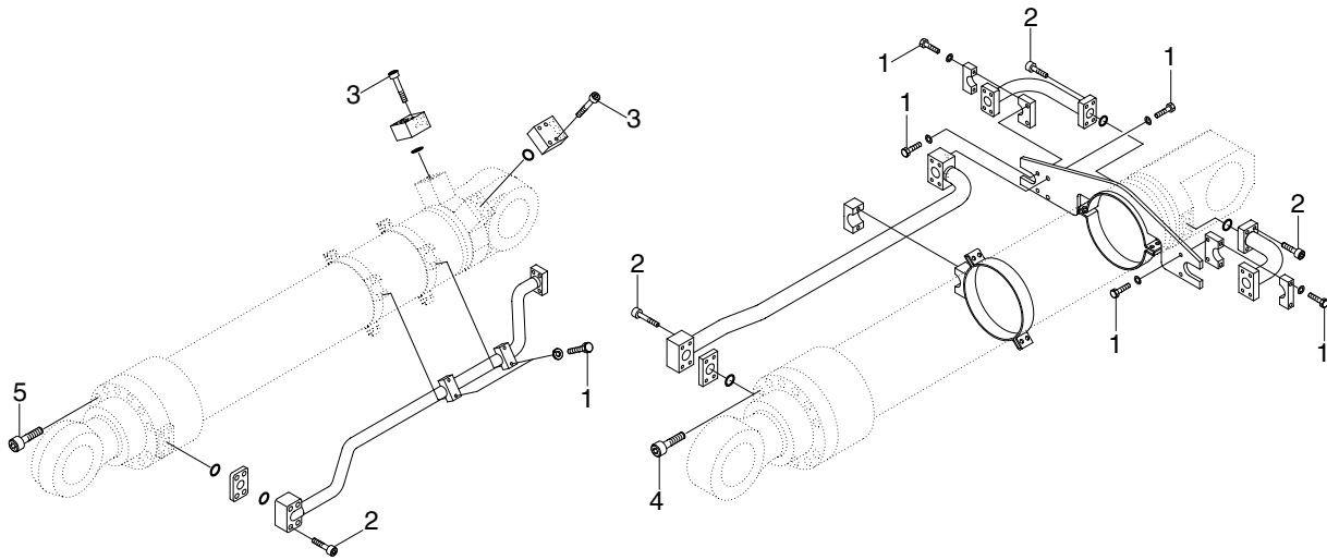
BOOM CYLINDER
