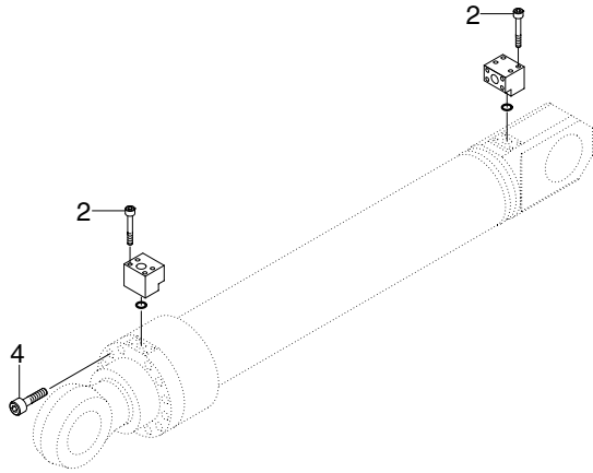
BOOM CYLINDER
