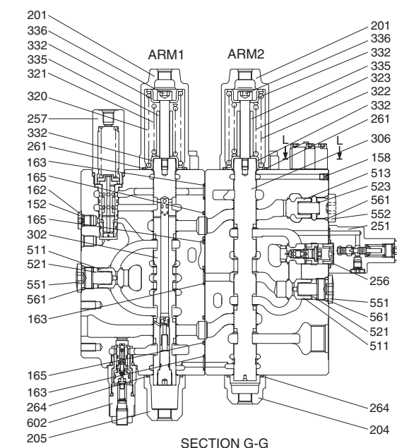
SECTION G-G
