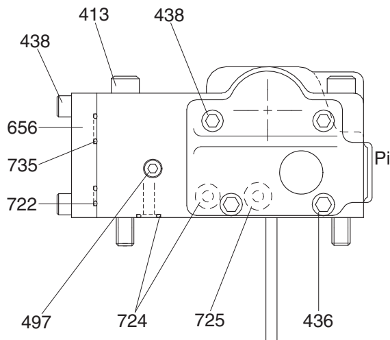
VIEW C
