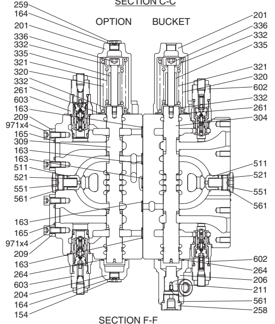
SECTION F-F
