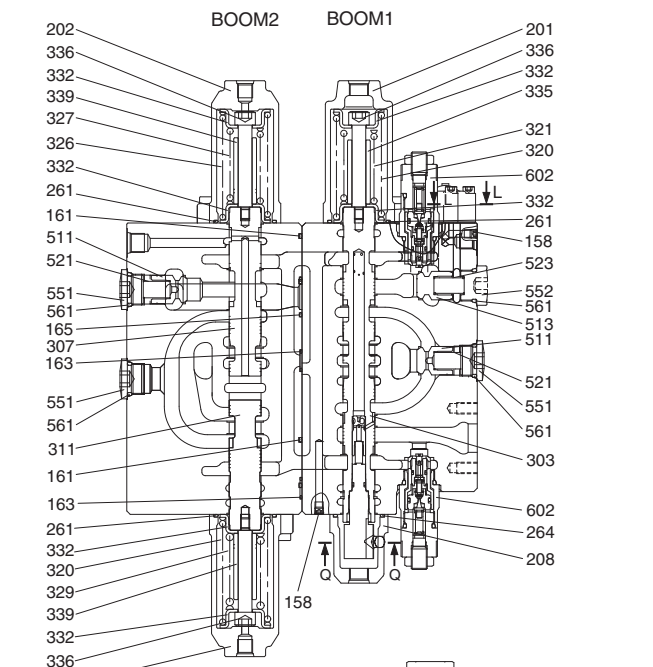
SECTION E-E
