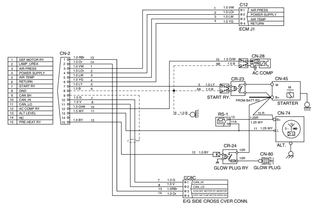
ENGINE HARNESS
