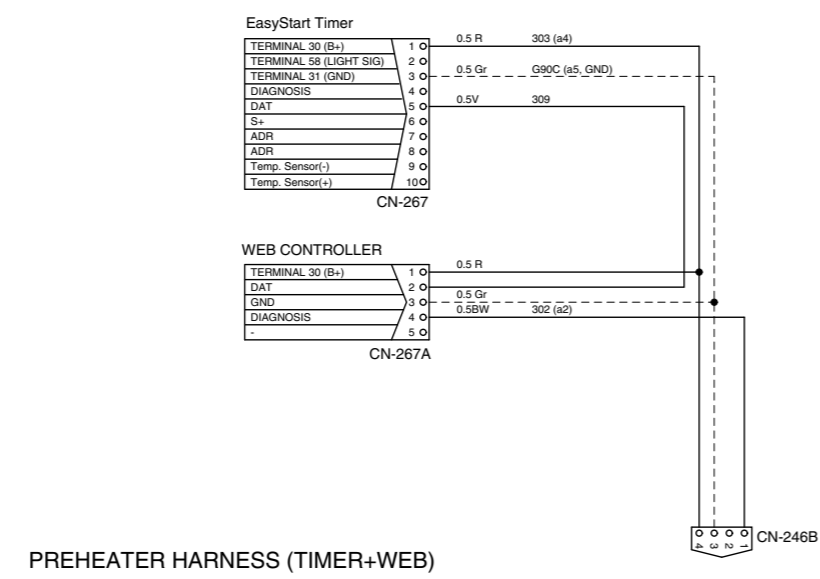
PREHEATER HARNESS (TIMER+WEB)
