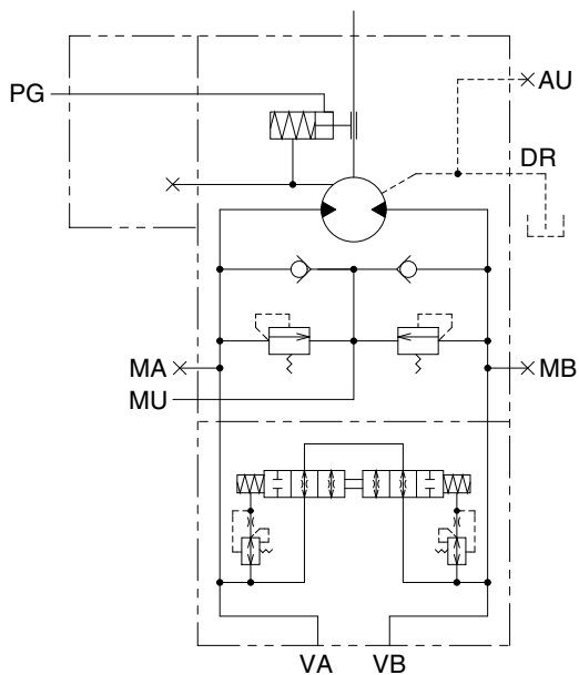
Hydraulic circuit
