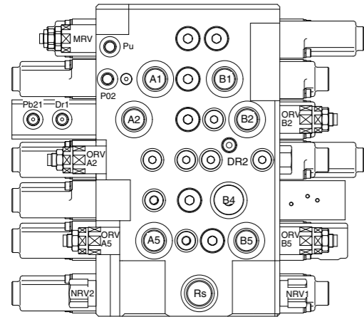
VIEW A
