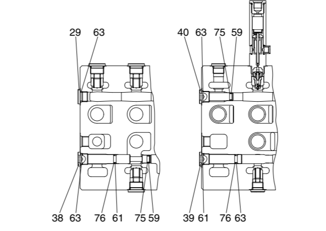
SECTION I-I
