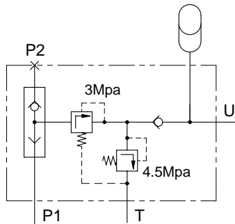
HYDRAULIC CIRCUIT
