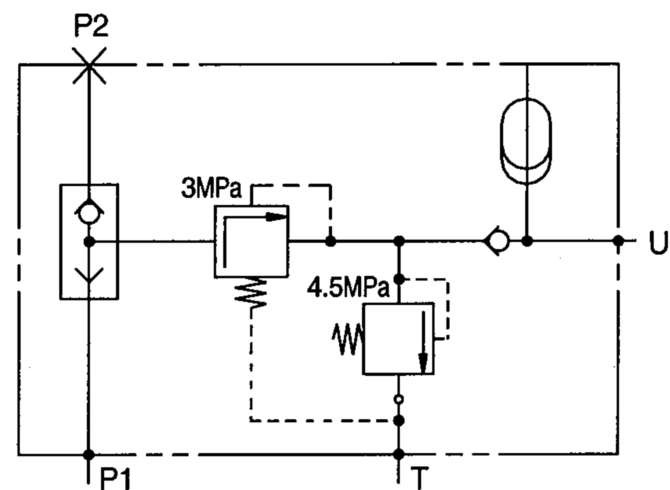
CIRCUIT DIAGRAM
