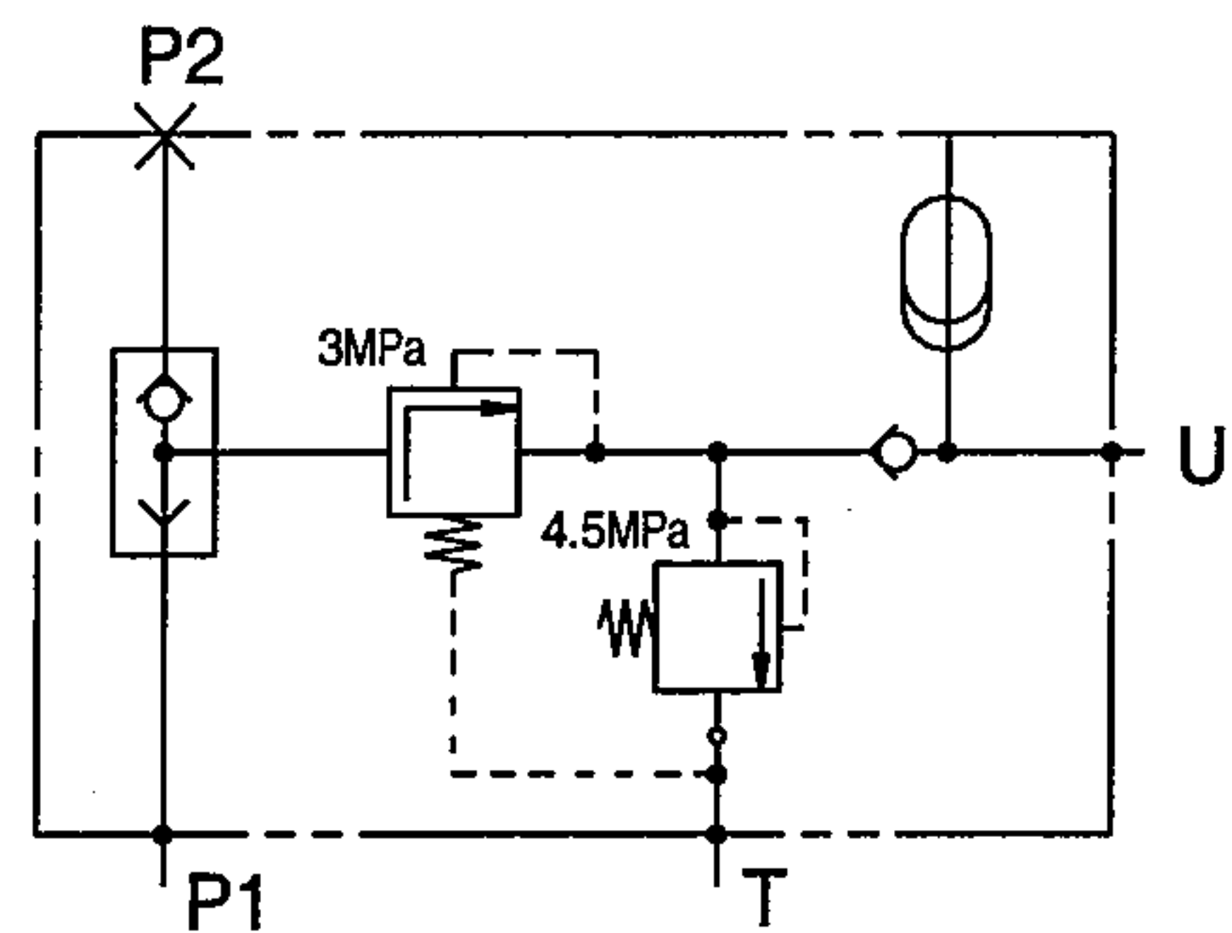
CIRCUIT DIAGRAM
